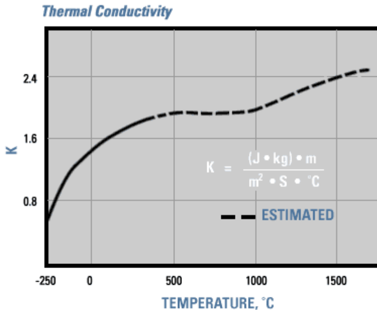
Representative thermal conductivity of fused quartz. Source: Published manufacturer's data.
